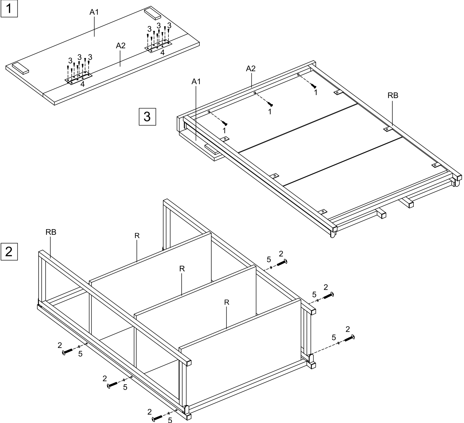
FINAL ASSEMBLING
