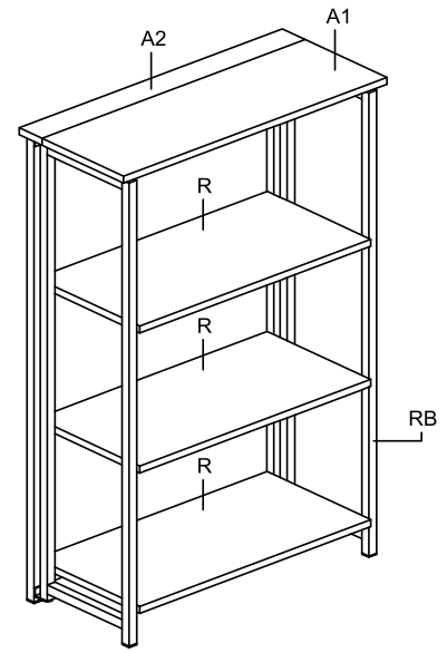
FINAL ASSEMBLING
